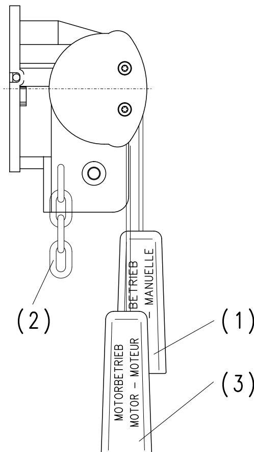
Fig. 1: Noodhandbediening "Snelle-Ketting"
